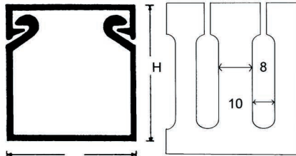
*SLOT DIMENTION APPLIES TO THE SLOTTED DUCT ONLY
